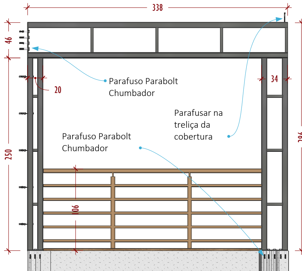
VISTA FRONTAL
