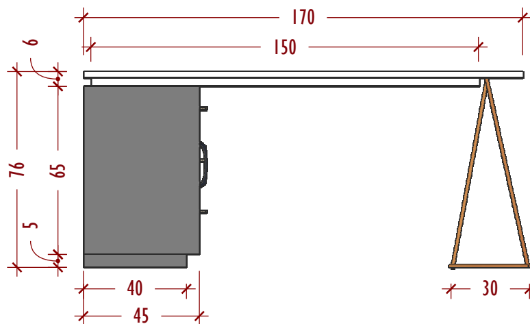
VISTA FRONTAL
