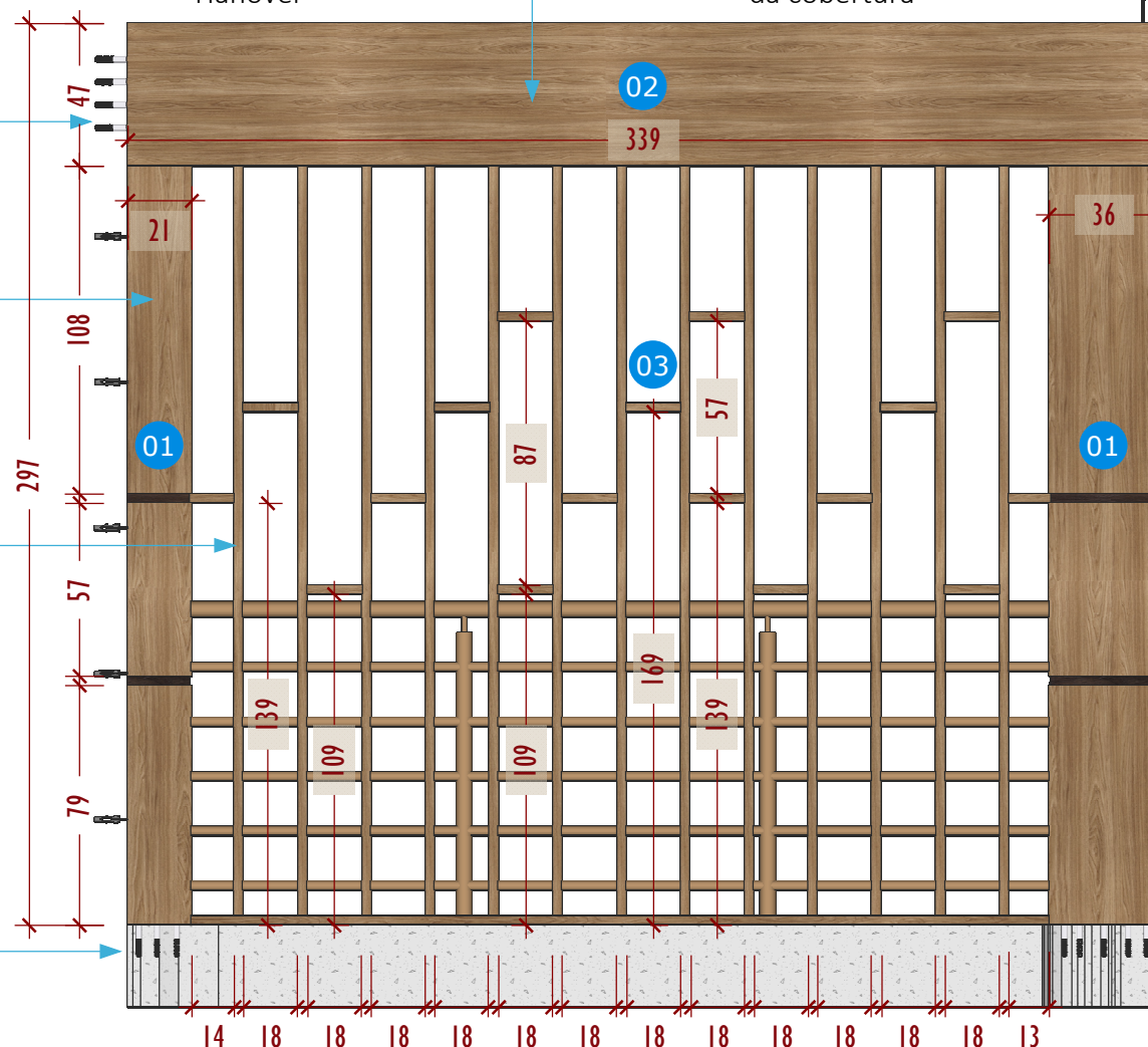
VISTA FRONTAL
